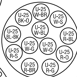
300 PAIR SUPER-UNIT
